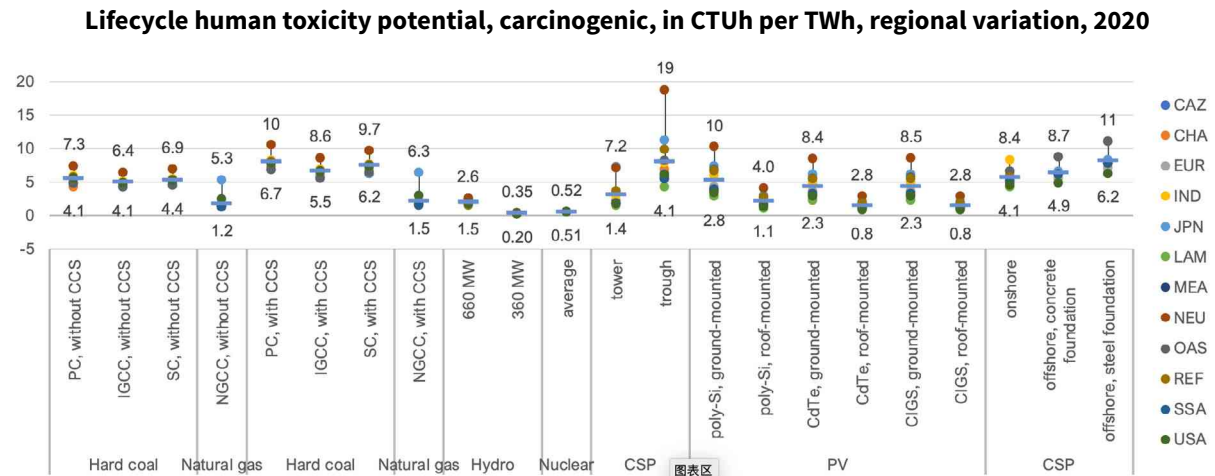
Figure 42 Lifecycle human toxicity (carcinogenic)' regional variations for year 2020. Variability is explained by several factors: electricity mix (all regions), region of extraction (fossil fuels), load factors (renewables). Nuclear power is modelled as a global average except for front-end.
