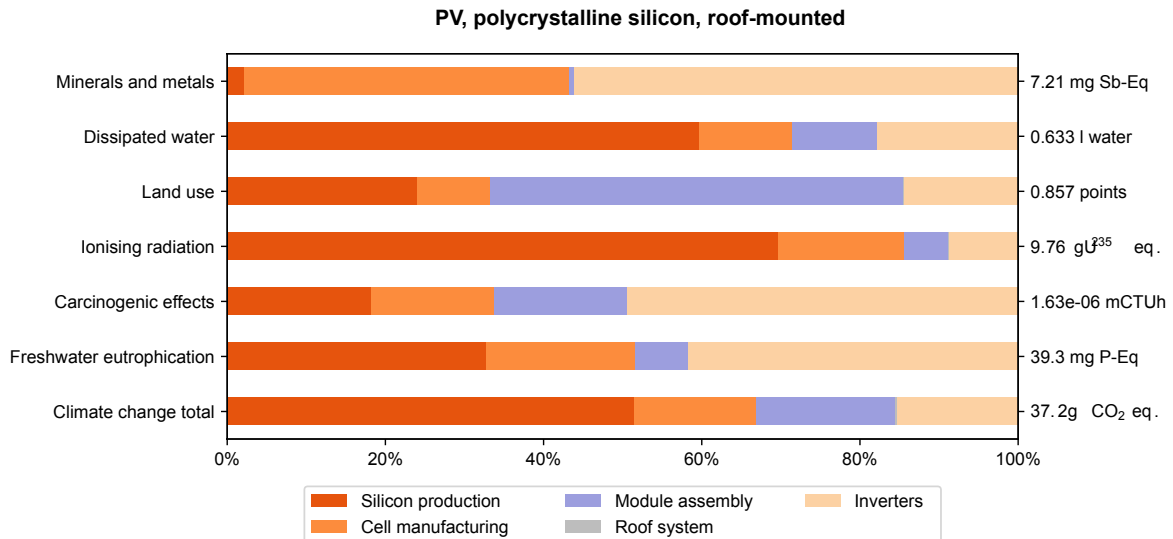
Figure 26 Life cycle impacts from 1 kWh of poly-Si, roof-mounted, photovoltaic power production, Europe, 2020
