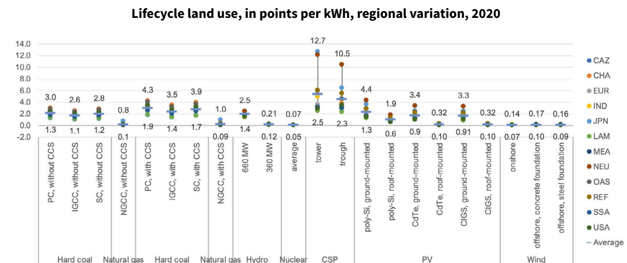
Figure 43 Lifecycle land use regional variations for year 2020. Variability is explained by several factors: electricity mix (all regions), methane leakage rates (fossil fuels), load factors (renewables). Nuclear power is modelled as a global average except for back-end.
