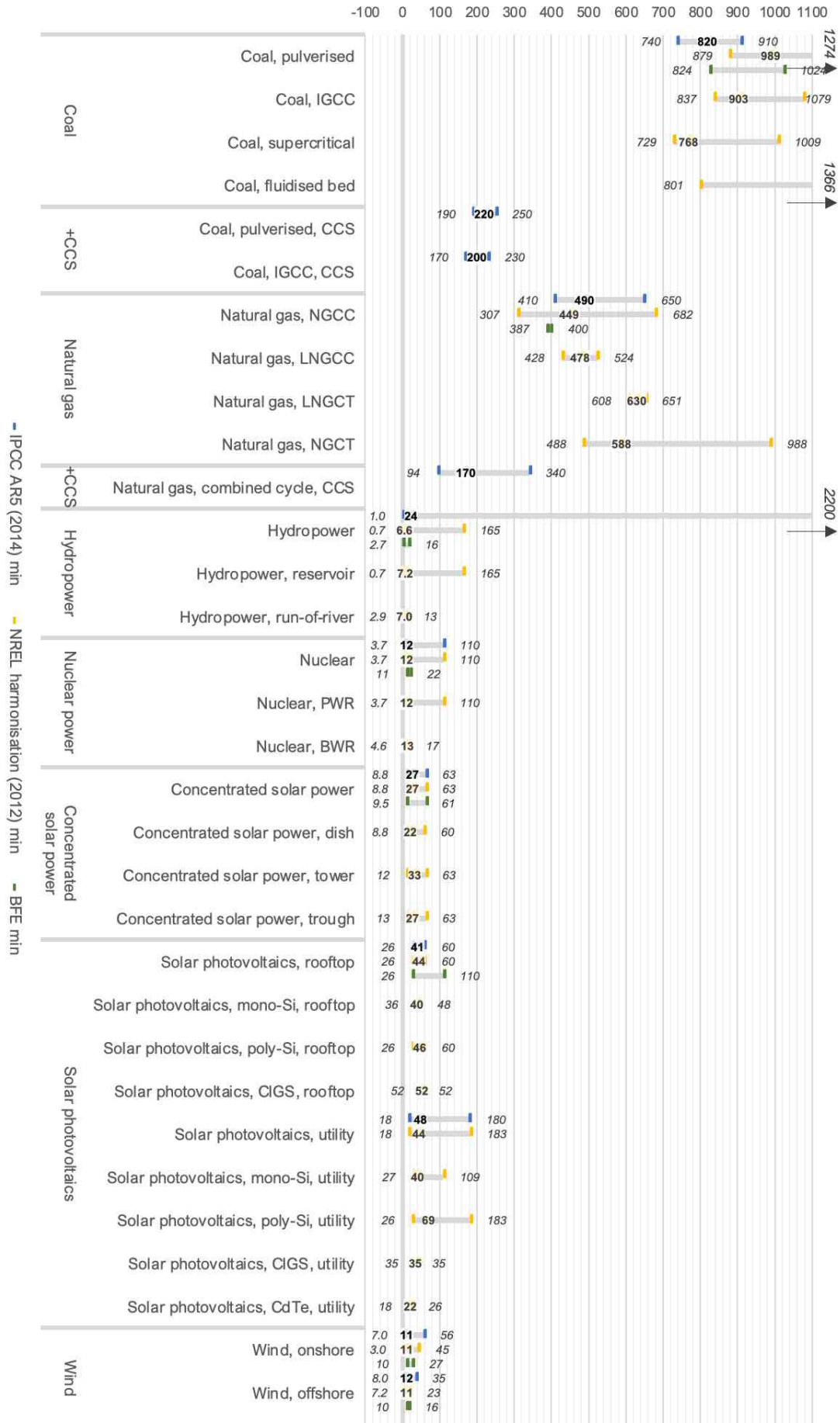
Lifecycle greenhouse emissions comparison of select electricity-generating technologies, in g CO 2 eq./kWh delivered to the grid
